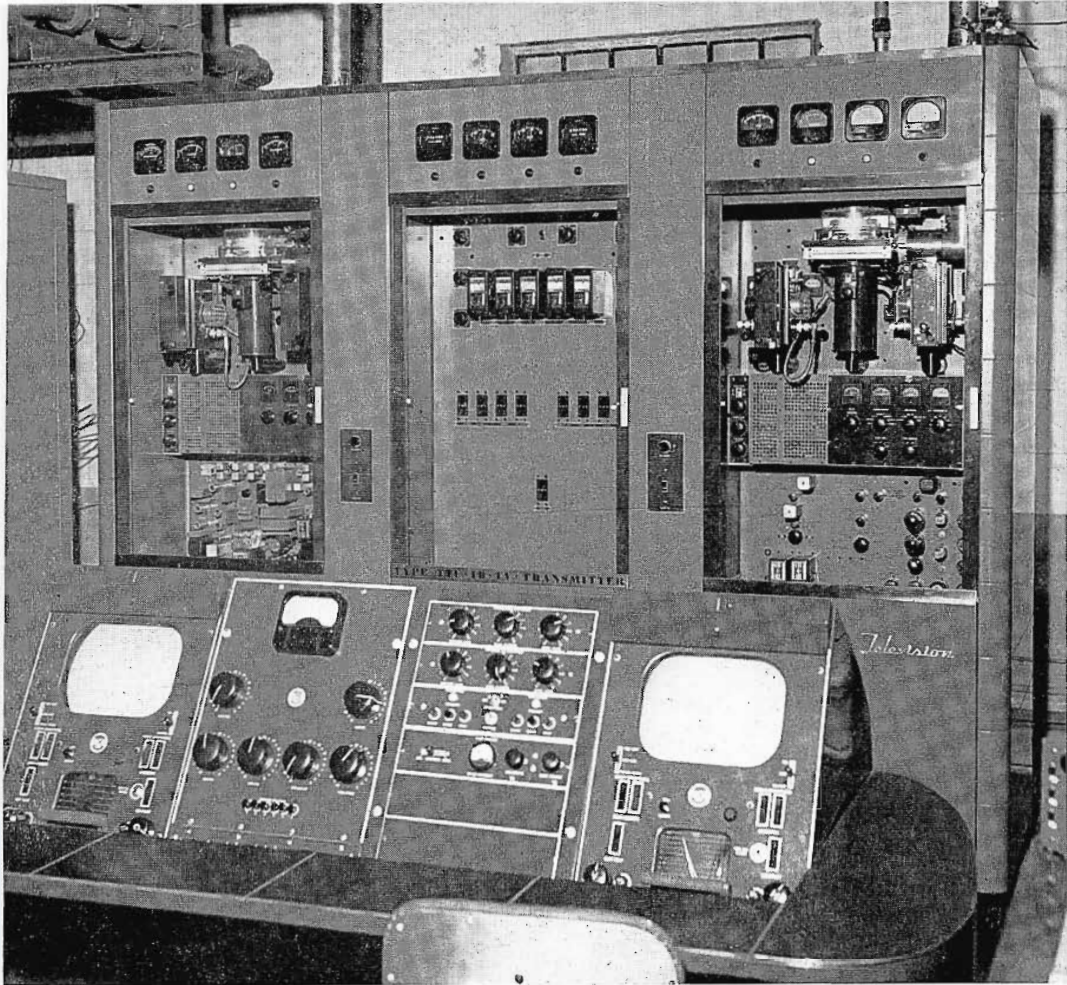
FIG. 4. Closeup of the RCA TTU-1B UHF television transmitter and TC-4A "Basic Buy" console—two excellent performers for UHF television broadcasting.
