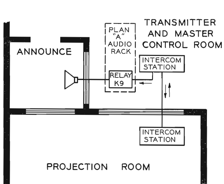
FIG. 16. Diagram showing the provision in Plan "A" for intercommunication facilities.
