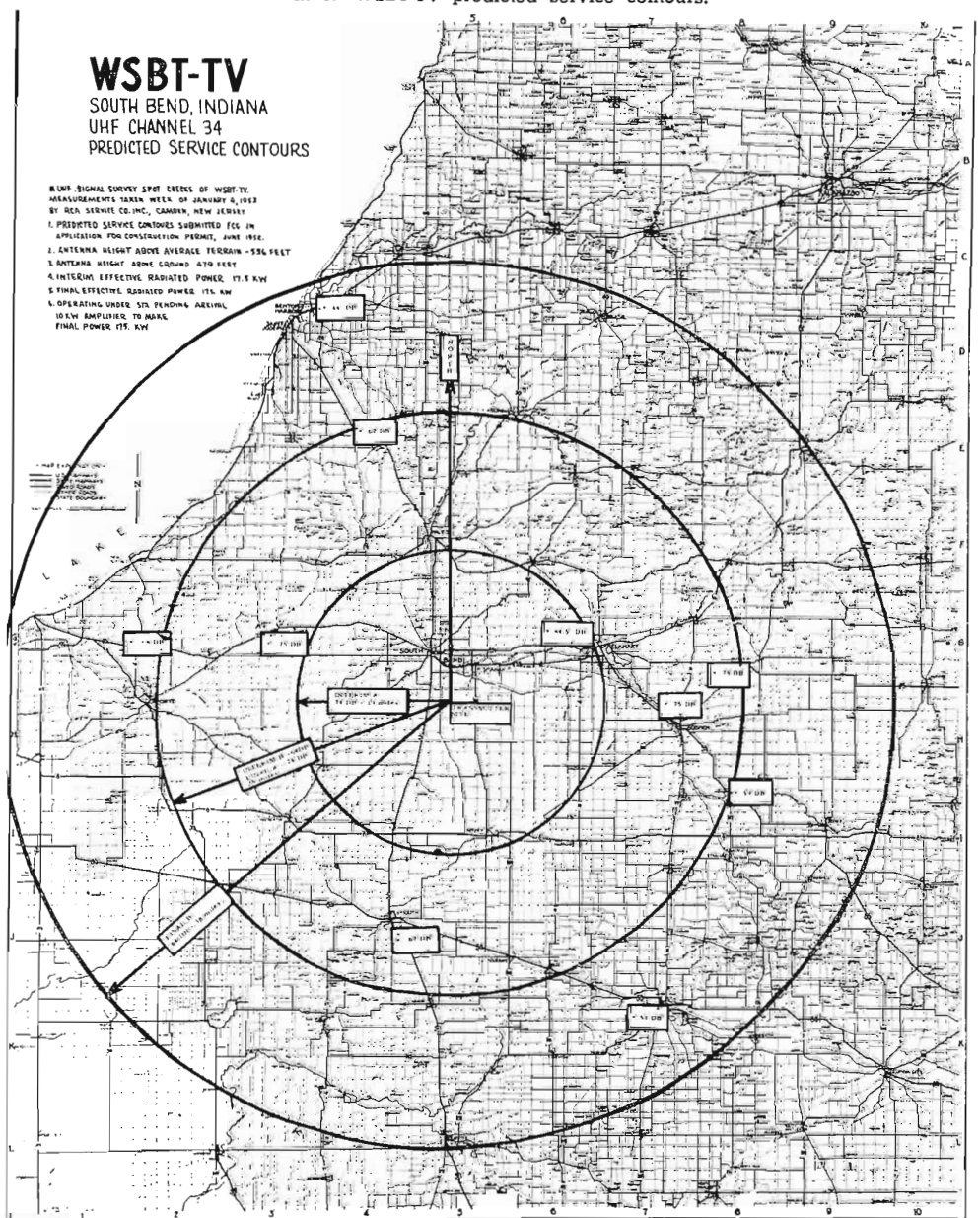
FIG. 9. WSBT-TV predicted service contours.
