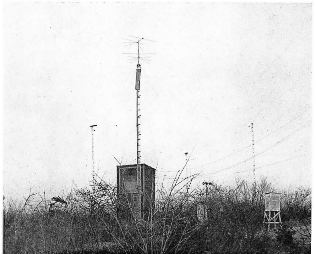
FIG. 9. Over-all view of Pimple Hill receiving point showing Rhombic antenna for WNBC and auxiliary antennas for Philadelphia. Site is also weather observation point for State Conservation Project.
