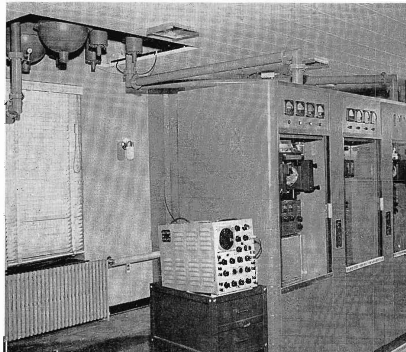
FIG. 4. View of the transmitter room. The transmitter plenum is not yet in place although the exhaust ducts may be seen. Note that the coax from the filterplexer may be swung to the right and left to meet the 10-KW amplifiers when delivered.
