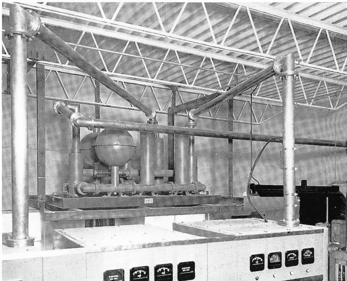
FIG. 5. Filterplexer arrangement as it is suspended from ceiling of WKNB-TV transmitter building.
