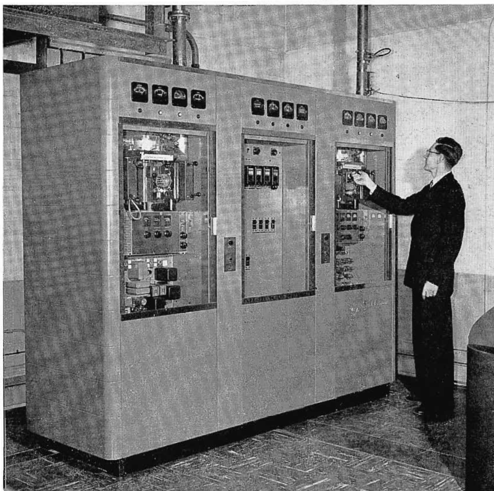
FIG. 1. Blair Thron, Vice-President and Director of Operations WFPG-TV, adjust cavity in visual section of the RCA TTU-1B UHF transmitter.
