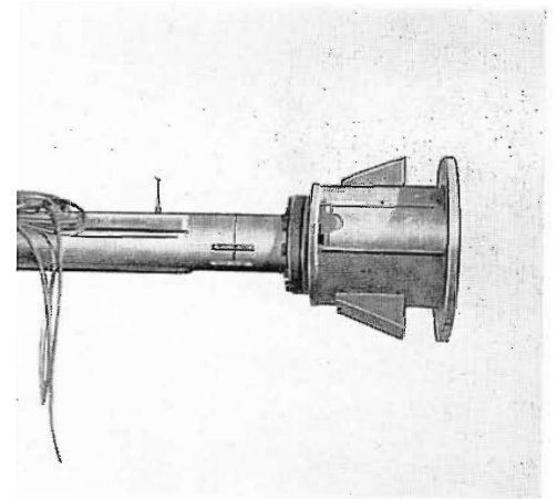
FIG. 10. Side view of Flange Pedestal Adapter fastened to base of UHF Pylon. Note hole in adapter near antenna base through which transmission line passes.
